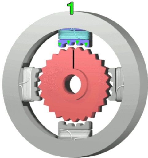
Figure 1.1. Stepper Motor
